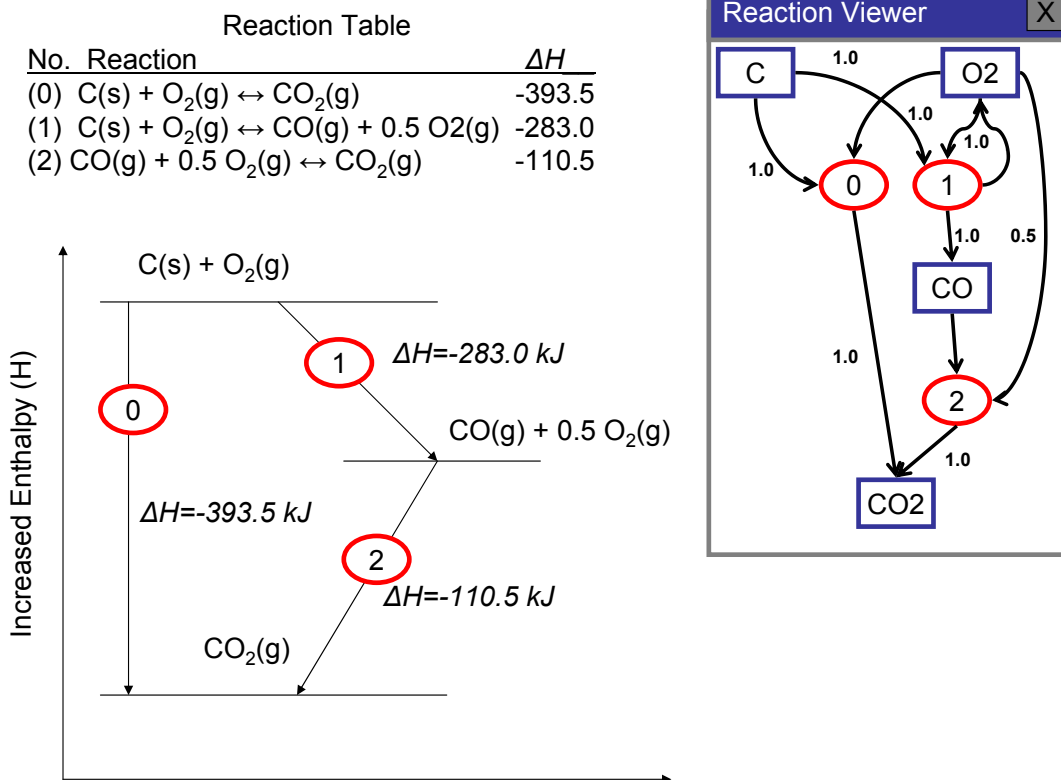
Figure 1: Enthalpy diagrams and thermochemical reaction tables.
